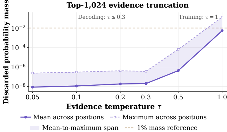
Figure 6: Probability mass discarded by top-1,024 evidence truncation. Mean and maximum backbone probability mass outside the retained candidates across 46,080 positions on LLaDA-1.0, as a function of evidence temperature \tau . Shading spans the mean and maximum; the horizontal dashed line marks 1% mass. At the training temperature \tau = 1 , the discarded mass averages 0.53% and reaches 13.2%. At the evaluated decoding temperatures \tau \leq 0.3 , the mean residual is numerically negligible, on the order of 10^{-8} .
