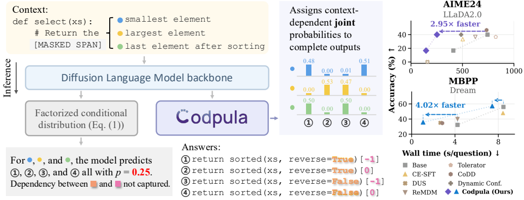
Figure 1: Factorized versus context-dependent joint prediction. Left: Given a masked return statement, a factorized denoiser predicts the sorting flag and index independently, assigning equal probability to all four completions regardless of the comment. Middle: Codpula assigns context-dependent joint probabilities, placing its mass on the completions consistent with each comment. Right: Codpula improves accuracy–latency trade-offs, achieving 2.95\times and 4.02\times speedups at matched accuracy on AIME24 (LLaDA-2.0; Bie et al. (2025)) and MBPP (Dream; Ye et al. (2025)).
