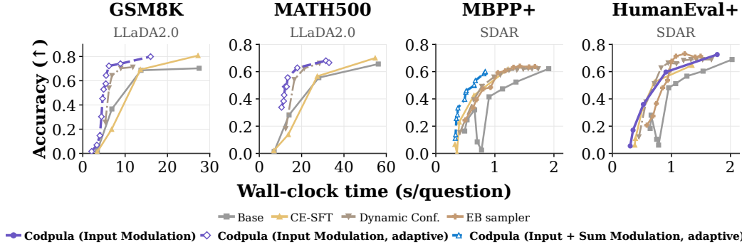
Figure 4: Accuracy-latency trade-offs on LLaDA-2.0 and SDAR. Accuracy versus wall-clock time per question for Codpula with uniform and adaptive decoding, base backbone, dynamic-confidence, and EB-sampler decoding on math (LLaDA-2.0) and code (SDAR) benchmarks.
