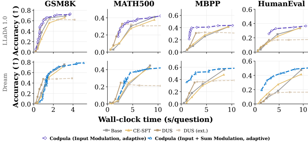
Figure 3: Accuracy-latency trade-offs on LLaDA-1.0 and Dream. Accuracy versus wall-clock time per question for adaptive Codpula, the base backbone, and DUS on math and code benchmarks.
