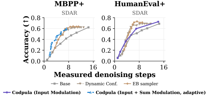
Figure 5: SDAR Accuracy versus Denoising Steps per Block. Accuracy on MBPP+ and HumanEval+ as a function of the mean measured number of denoising steps per block. The results use the same evaluation settings as the SDAR panels in Figure 4. This view complements the runtime comparison by separating per-block denoising effort from the number of blocks generated before early stopping.
