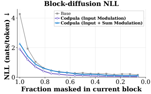
Figure 2: Block-diffusion NLL on Dream. Negative log-likelihood (nats/token) versus the fraction of masked tokens in the current block. Both Codpula variants substantially reduce NLL when most of the block is masked.
