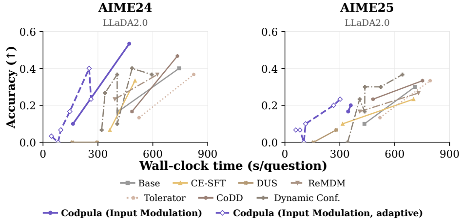
Figure 9: Accuracy–time trade-offs on AIME24 and AIME25. Results use LLaDA-2.0-mini. Codpula (Input Only) is evaluated with uniform decoding (solid purple) and dependence-adaptive decoding (dashed purple). Each marker denotes an evaluated decoding configuration; lines connect configurations of the same method.
