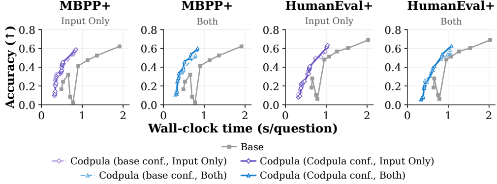
Figure 7: Confidence Source for Token Commitment. Accuracy–runtime trade-offs on MBPP+ and HumanEval+ for SDAR with Codpula (Input Only) and Codpula (Both). Both confidence variants use Codpula’s token proposals and dependence-based deferral, with candidate positions ranked using either backbone confidence ( base conf. ) or the refined distribution ( Codpula conf. ). The unmodified backbone is included as a reference.
