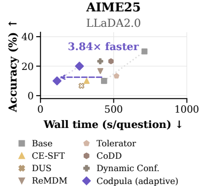
Figure 8: Additional AIME25 results with LLaDA-2.0-mini. Accuracy (%) versus wall-clock time per question. Adaptive Codpula achieves a 3.84\times speedup over the base model at matched 10% accuracy.
